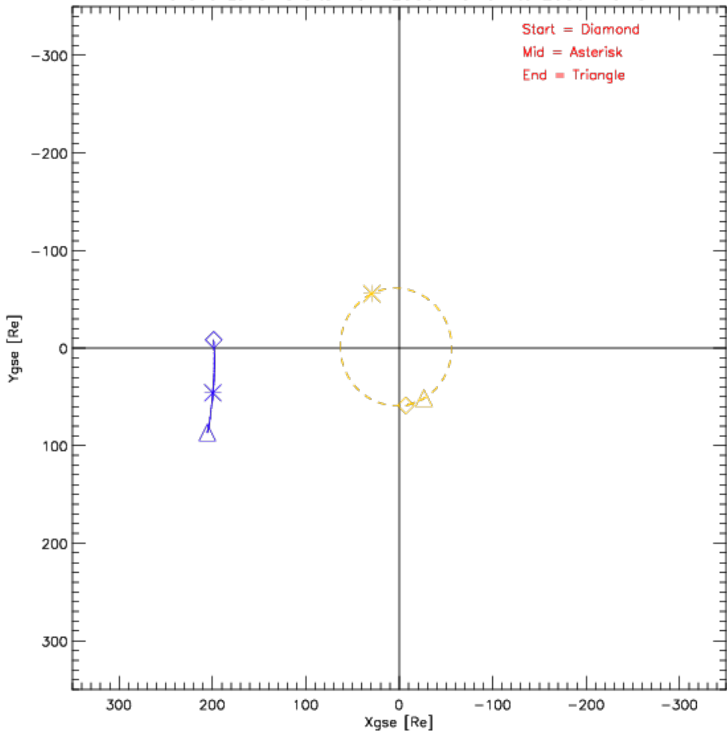
Wind and Lunar Orbits from 2006-10-01 to 2006-10-31
