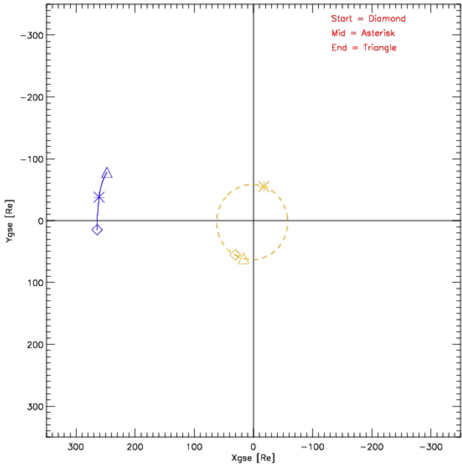
Wind and Lunar Orbits from 2006-07-01 to 2006-07-31
