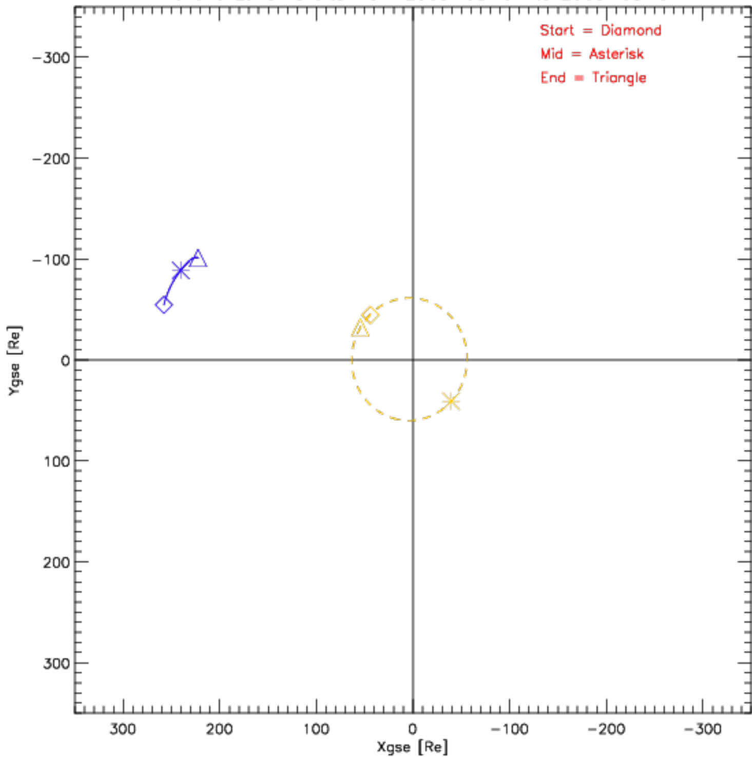
Wind and Lunar Orbits from 2005-08-01 to 2005-08-31
