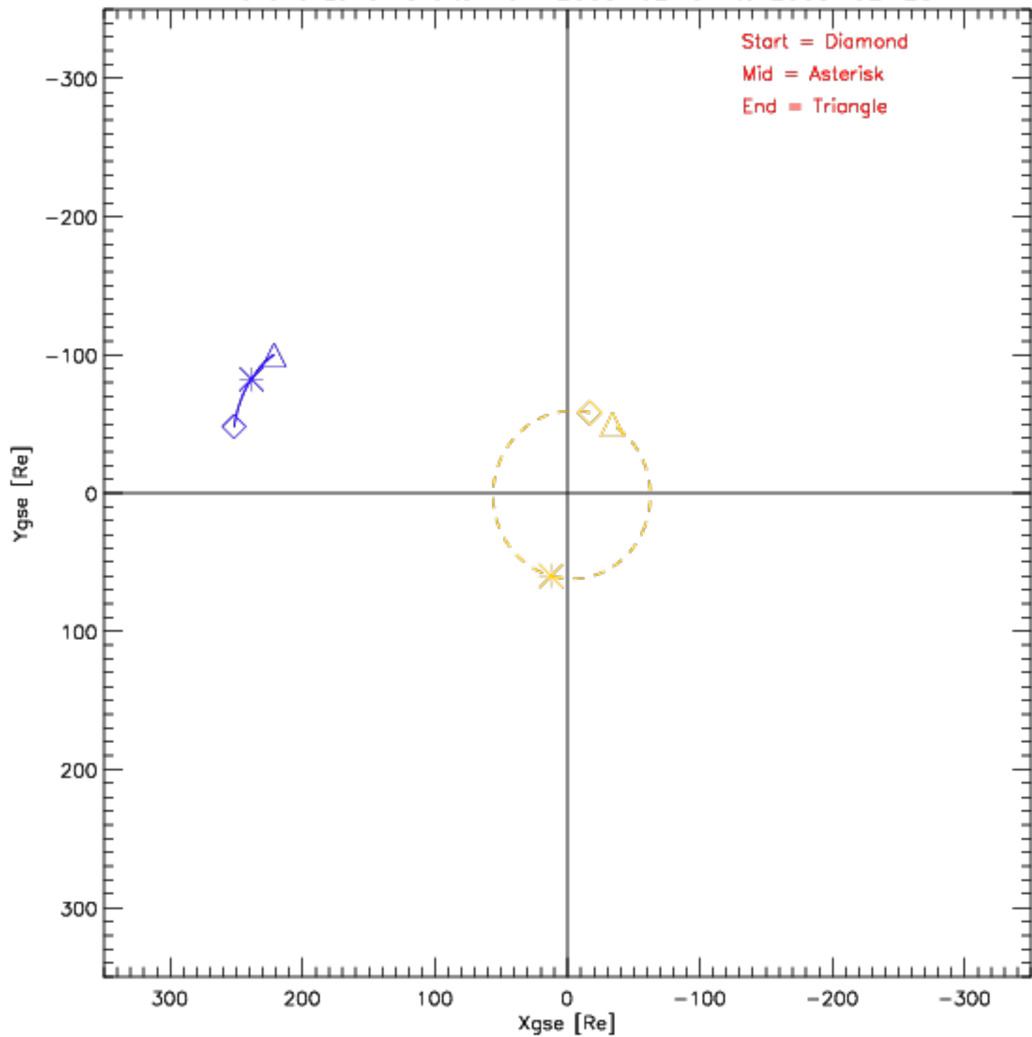
Wind and Lunar Orbits from 2005-02-01 to 2005-02-28
