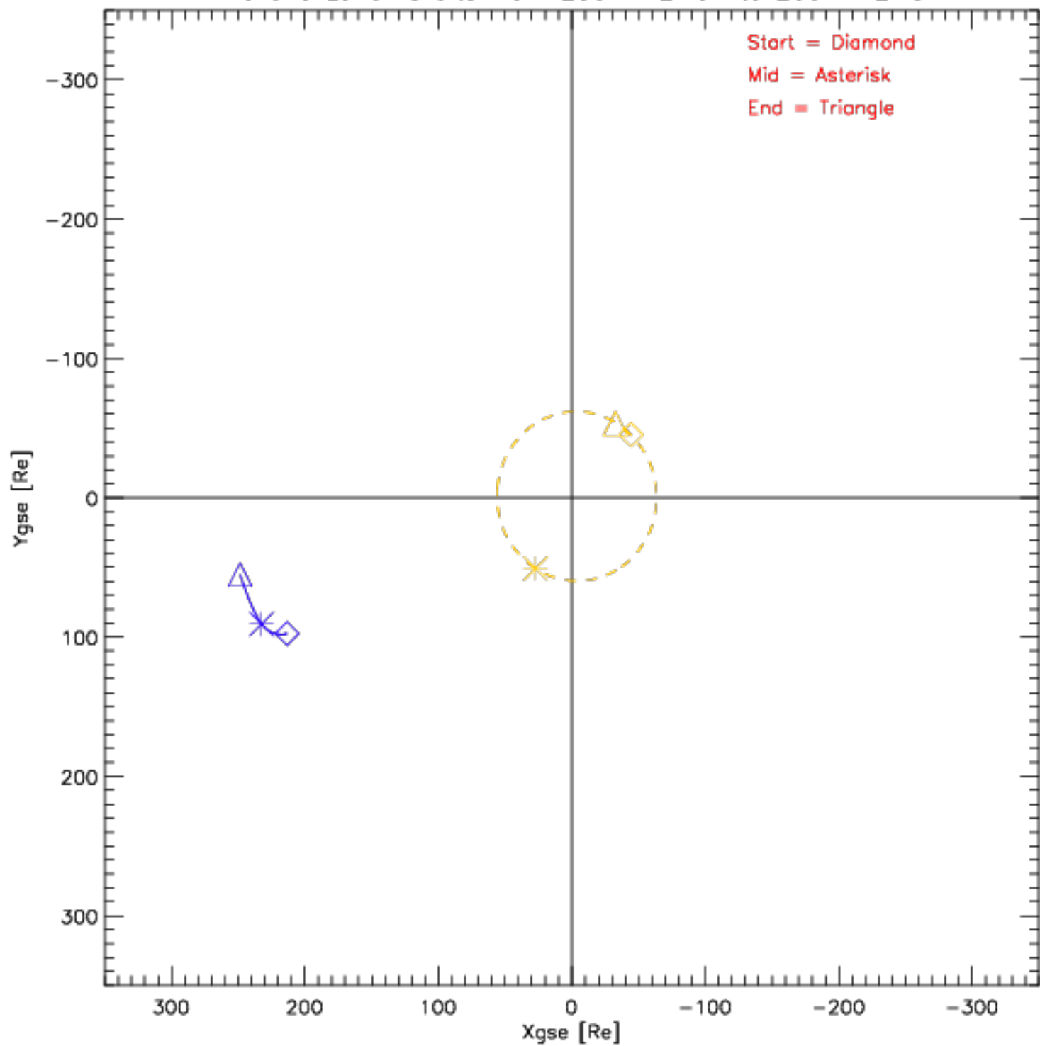
Wind and Lunar Orbits from 2004-12-01 to 2004-12-31
