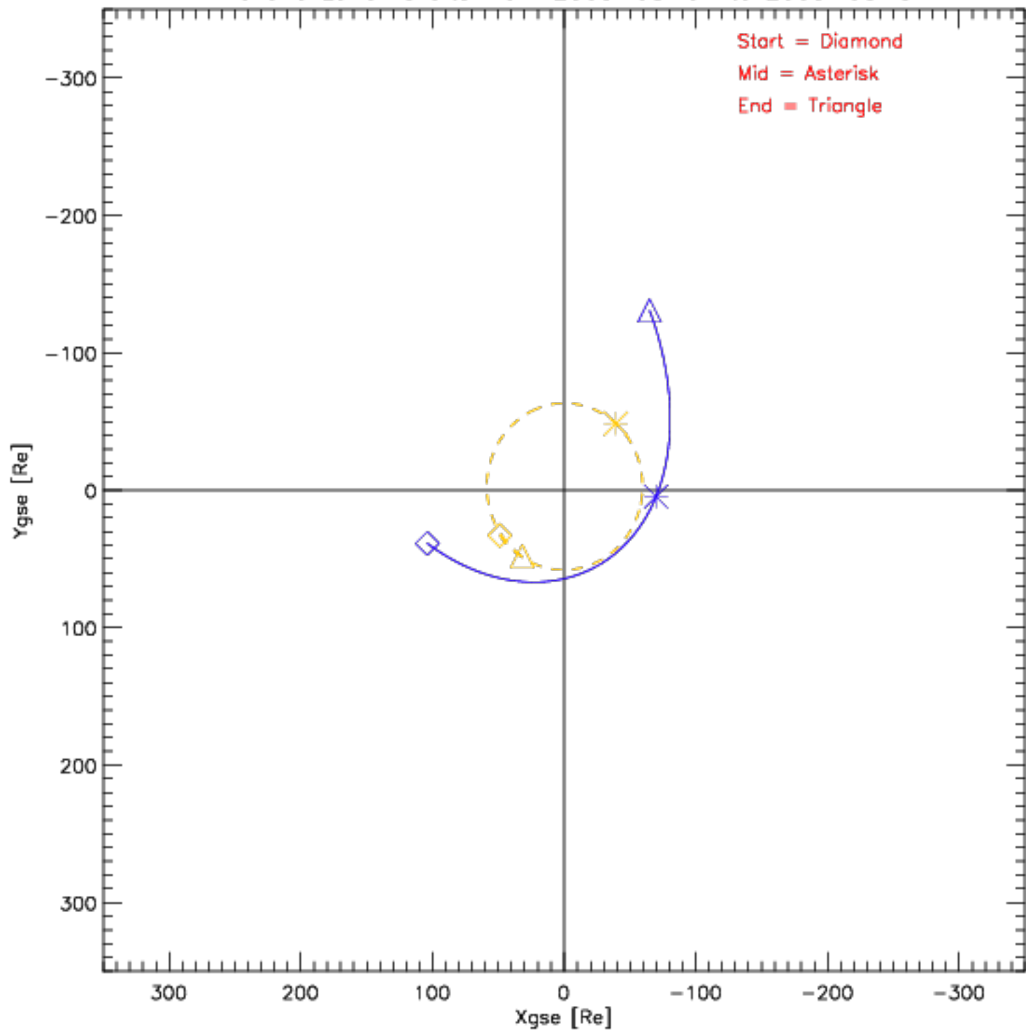
Wind and Lunar Orbits from 2003-08-01 to 2003-08-31
