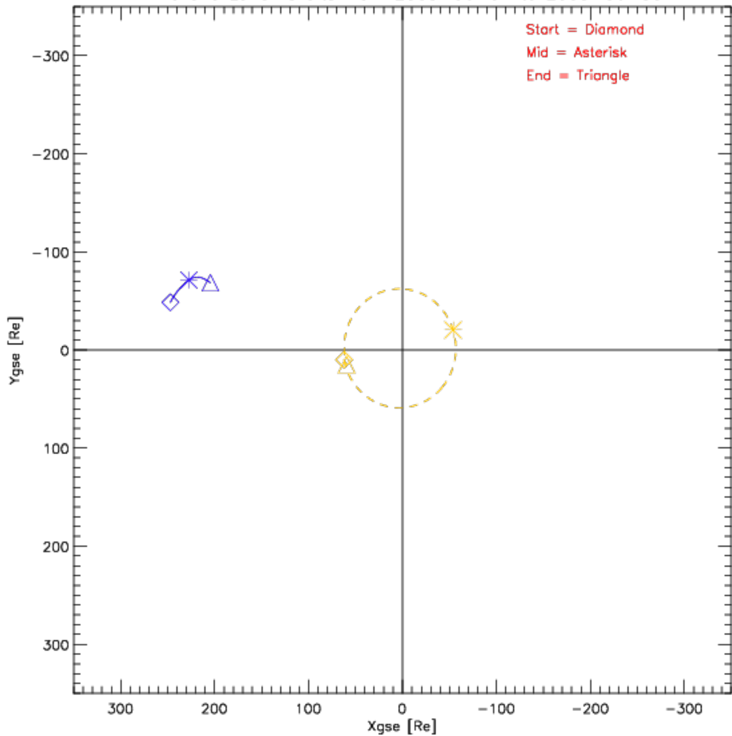
Wind and Lunar Orbits from 2003-06-01 to 2003-06-30
