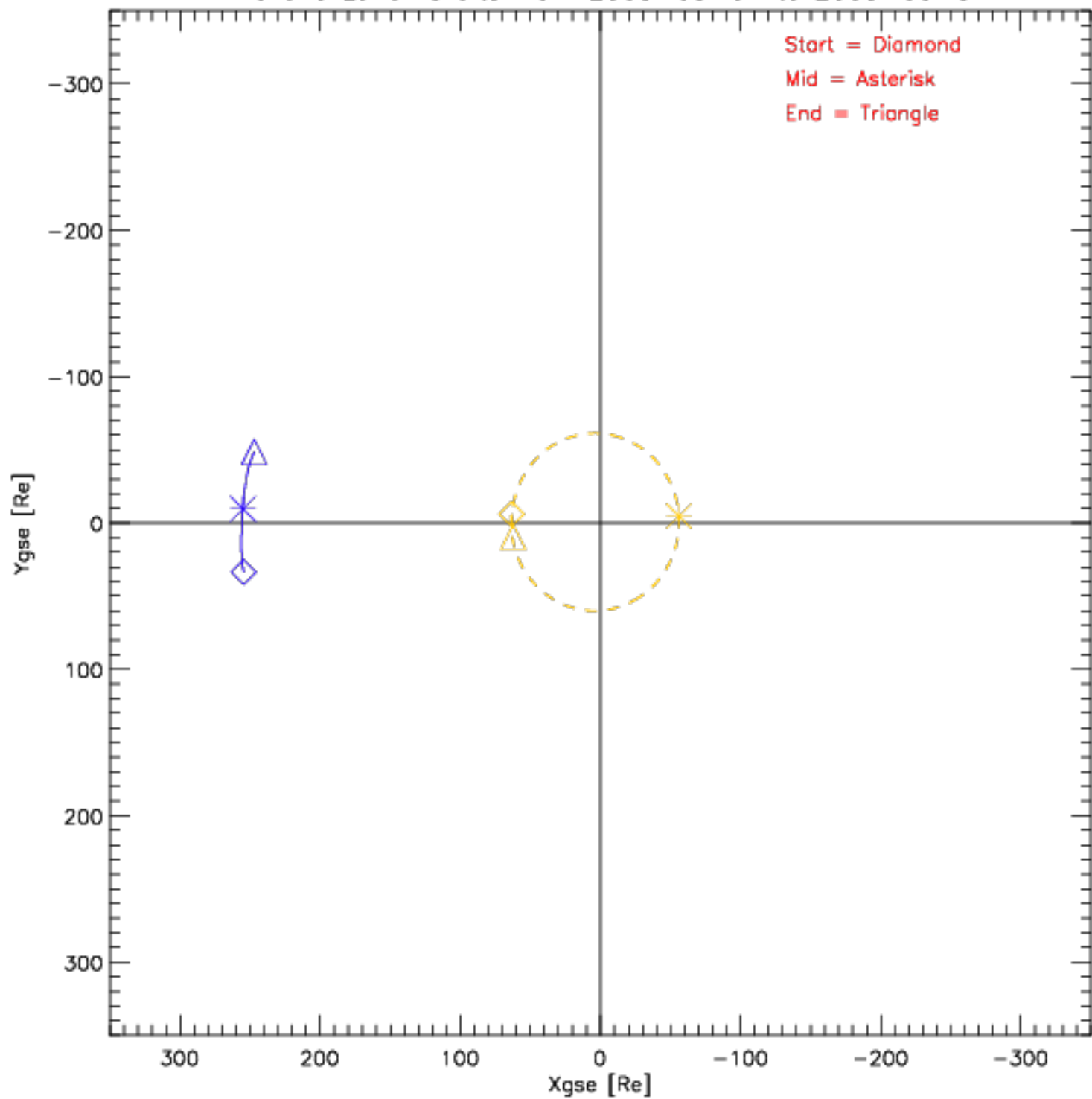
Wind and Lunar Orbits from 2003-05-01 to 2003-05-31
