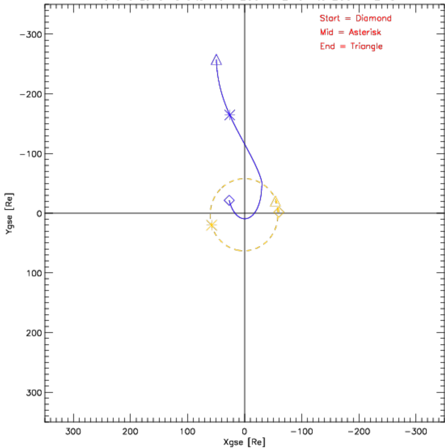
Wind and Lunar Orbits from 2001-12-01 to 2001-12-31
