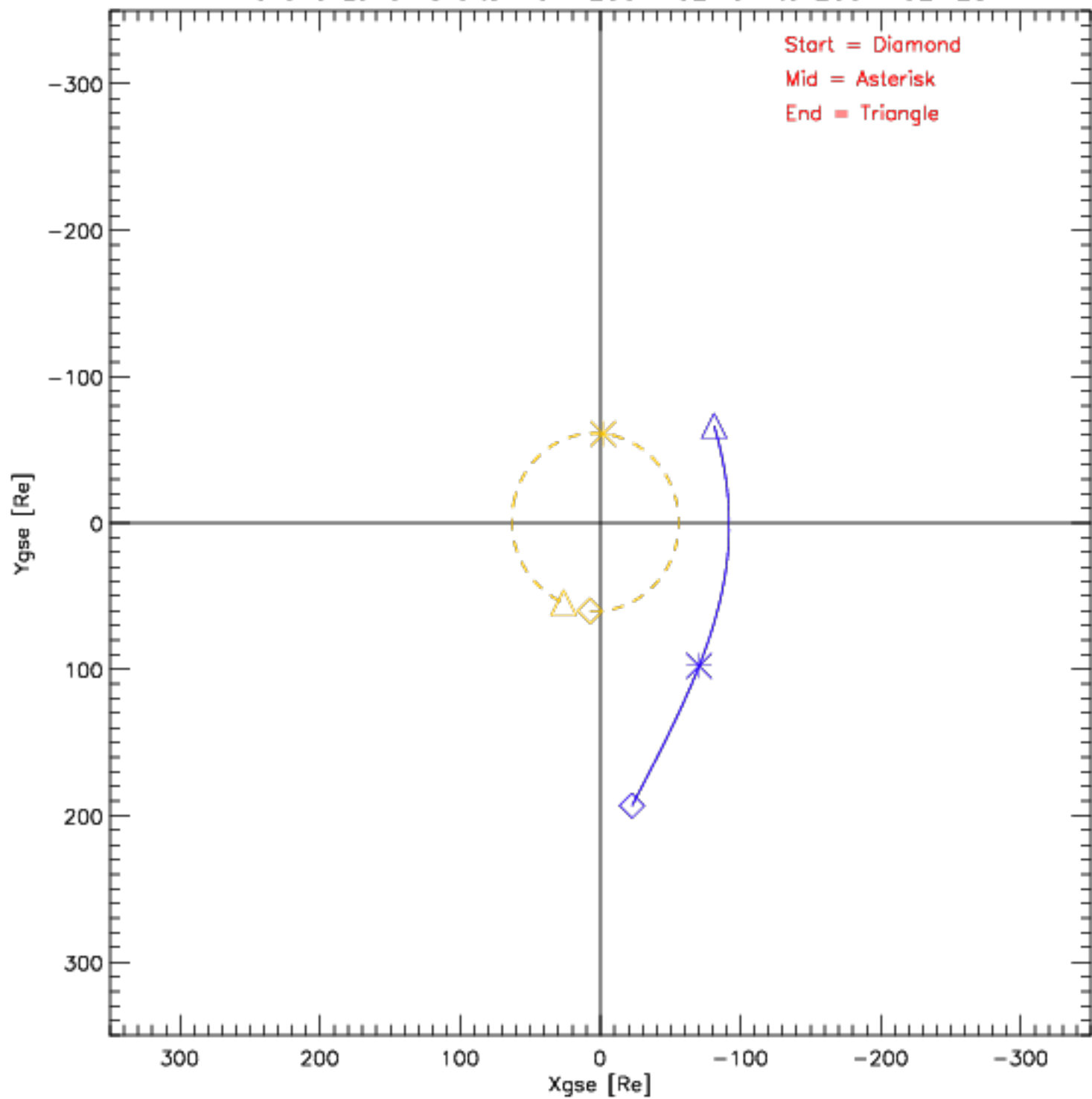
Wind and Lunar Orbits from 2001-02-01 to 2001-02-28
