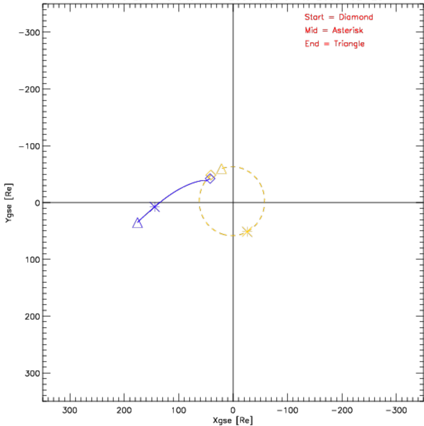
Wind and Lunar Orbits from 2000-02-01 to 2000-02-28
