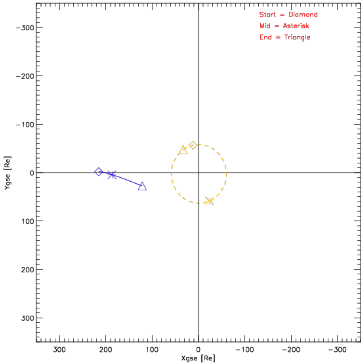
Wind and Lunar Orbits from 1997-05-01 to 1997-05-31
