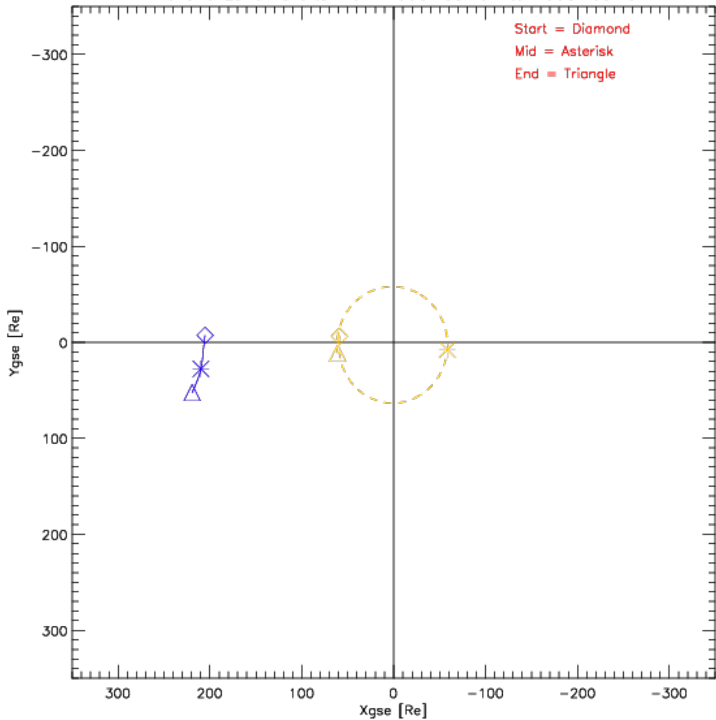
Wind and Lunar Orbits from 1995-03-01 to 1995-03-31
